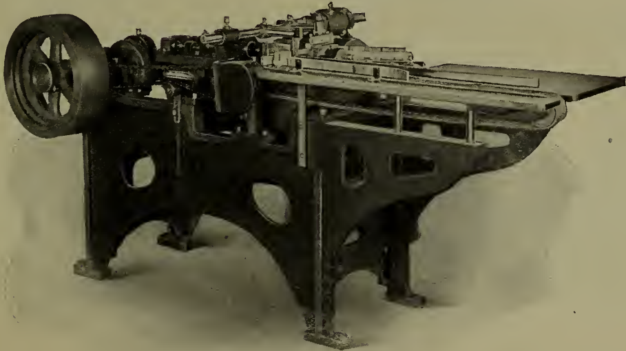
Style D Sheet Feed Wrapping Machine.
